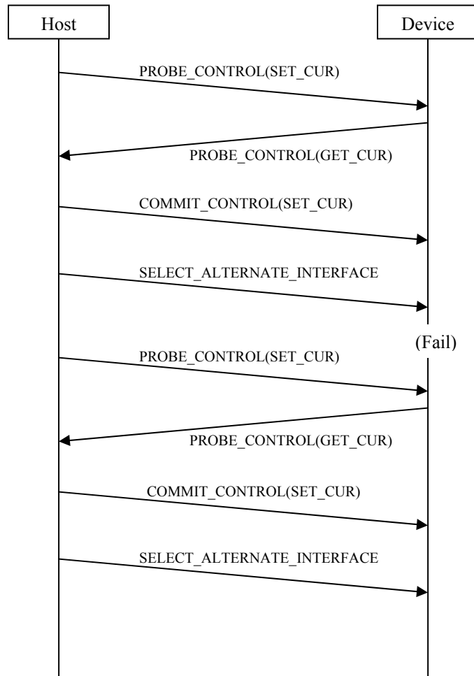
Figure 4-2 Failed USB Isochronous Bandwidth Negotiation
