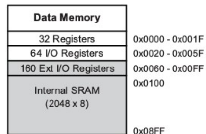
Figure 7-2. Data Memory Map
